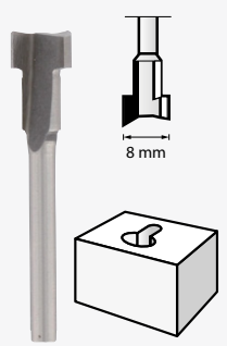
Router Bit (HSS) 8,0 mm (655)
