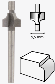
Router Bit (HSS) 9,5 mm (612)
