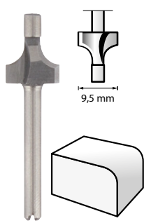
Router Bit (HSS) 9,5 mm (615)
