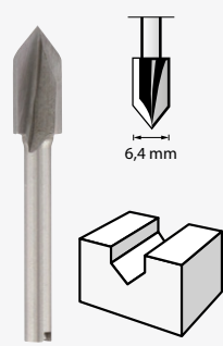
Router Bit (HSS) 6,4 mm (640)
