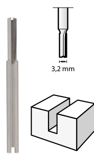
Router Bit (HSS) 3,2 mm (650)
