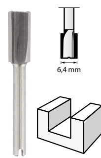
Router Bit (HSS) 6,4 mm (654)
